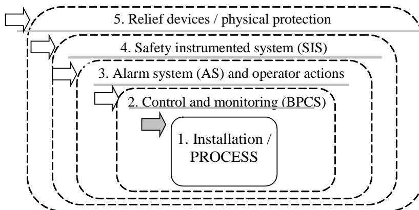
Figure 3. Typical protection layers in hazardous industrial installation
